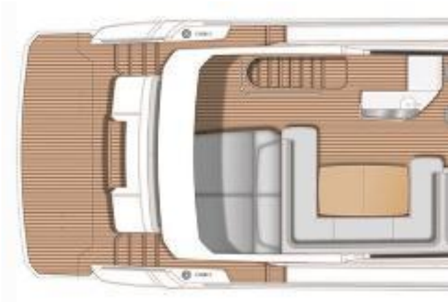
Manufacturer Provided Image: Princess F70 Flybridge Layout Plan
