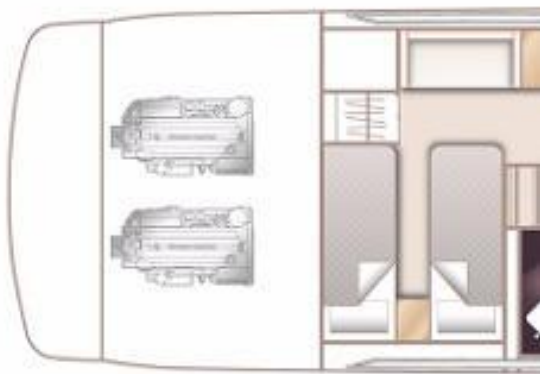
Princess V40 Lower Deck Layout Plan
