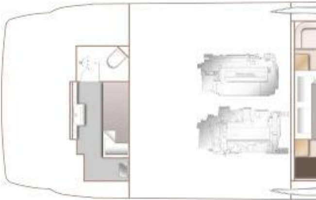
Manufacturer Provided Image: Princess 55 Lower Deck Layout Plan
