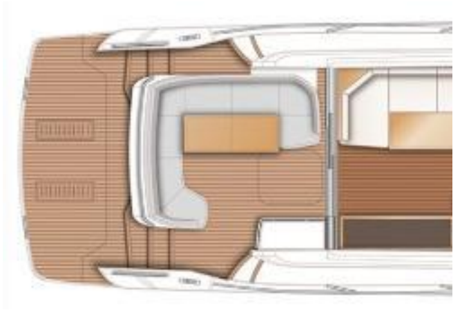
Princess V50 Main Deck Layout Plan
