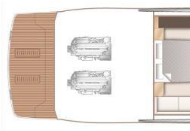
Princess V50 Lower Deck Layout Plan
