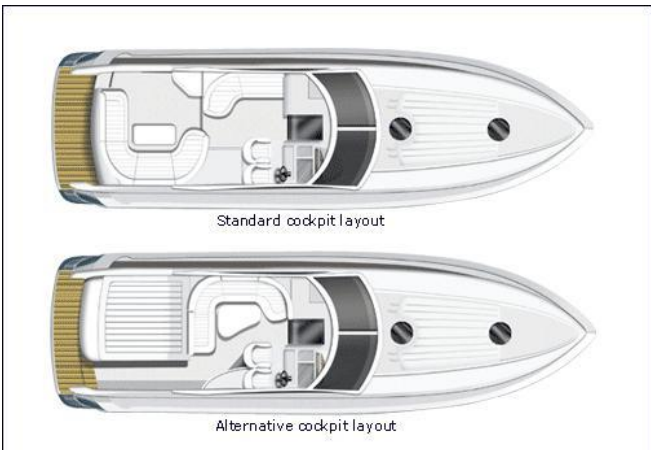
Manufacturer Provided Image: Floor Plans
